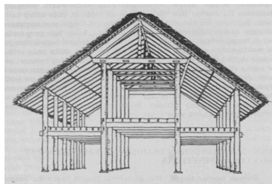
Figure 2. Traditional House Framework Seen from the Front [Source: Arsitektur Tradisional Provinsi Daerah Istimewa Aceh , 1981 page 26]
