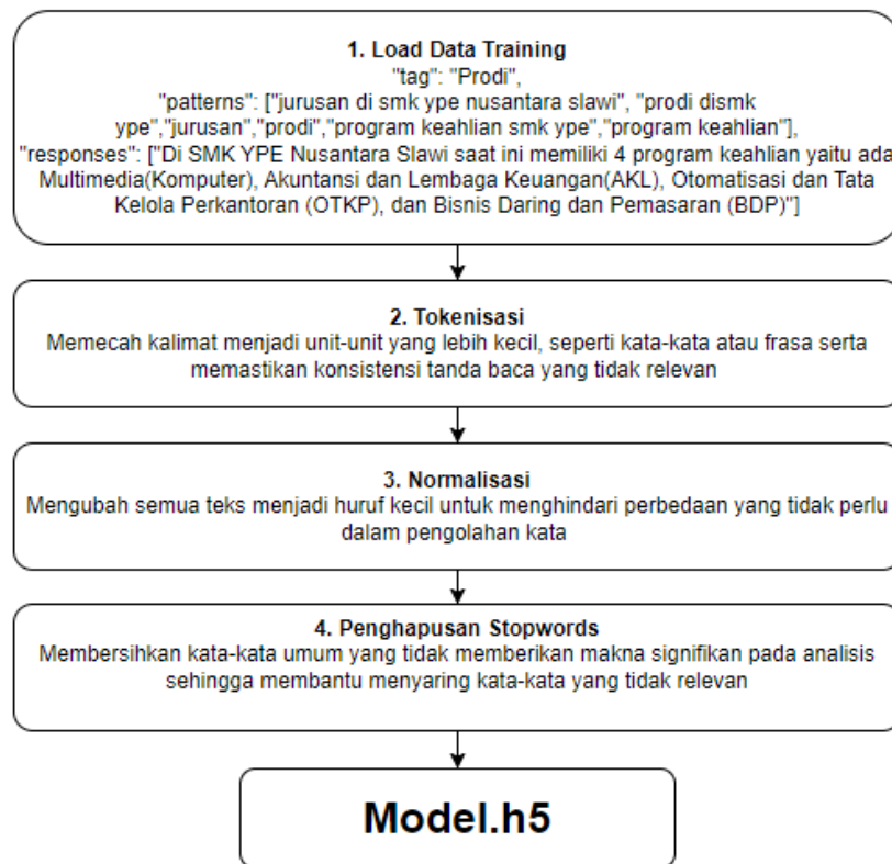
Gambar 3 Proses Data Training
